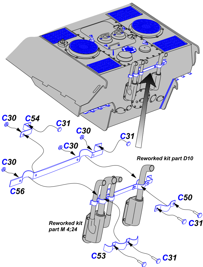
Panther version Ausf. A late/early
