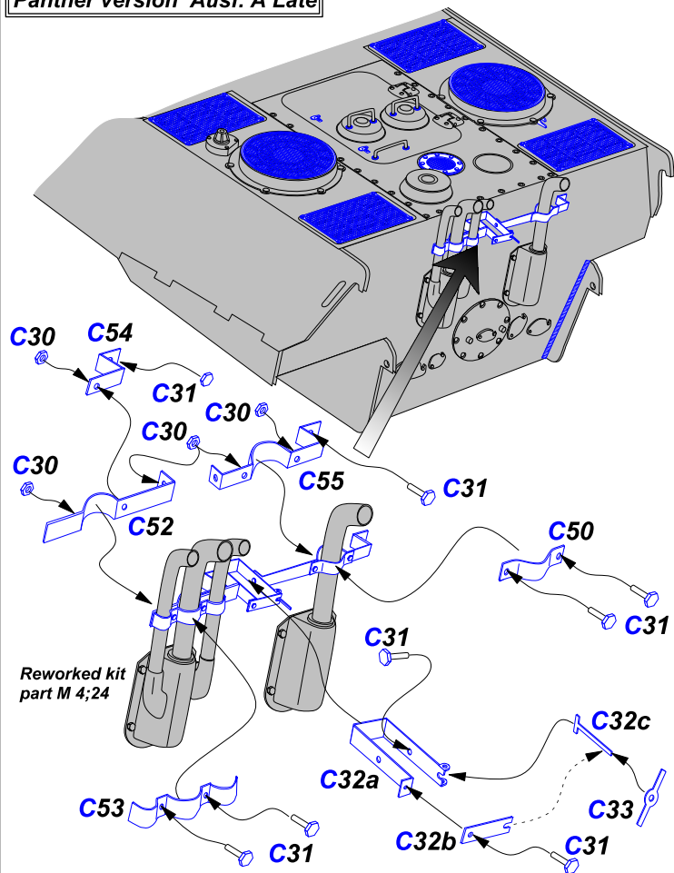
Panther version Ausf. A Late
