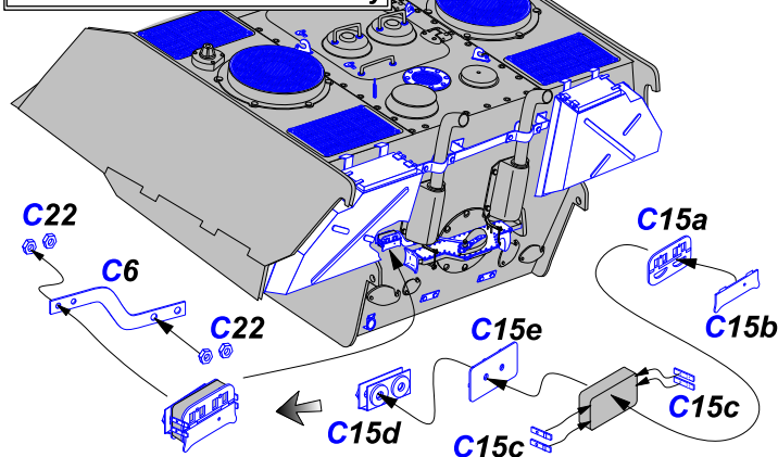
Panther version Ausf. A early
