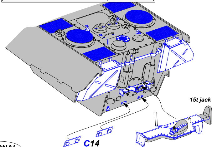
Panther version Ausf. A early Late model
